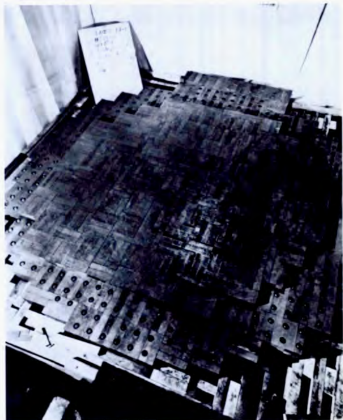
The chain-reacting pile at Chicago.
